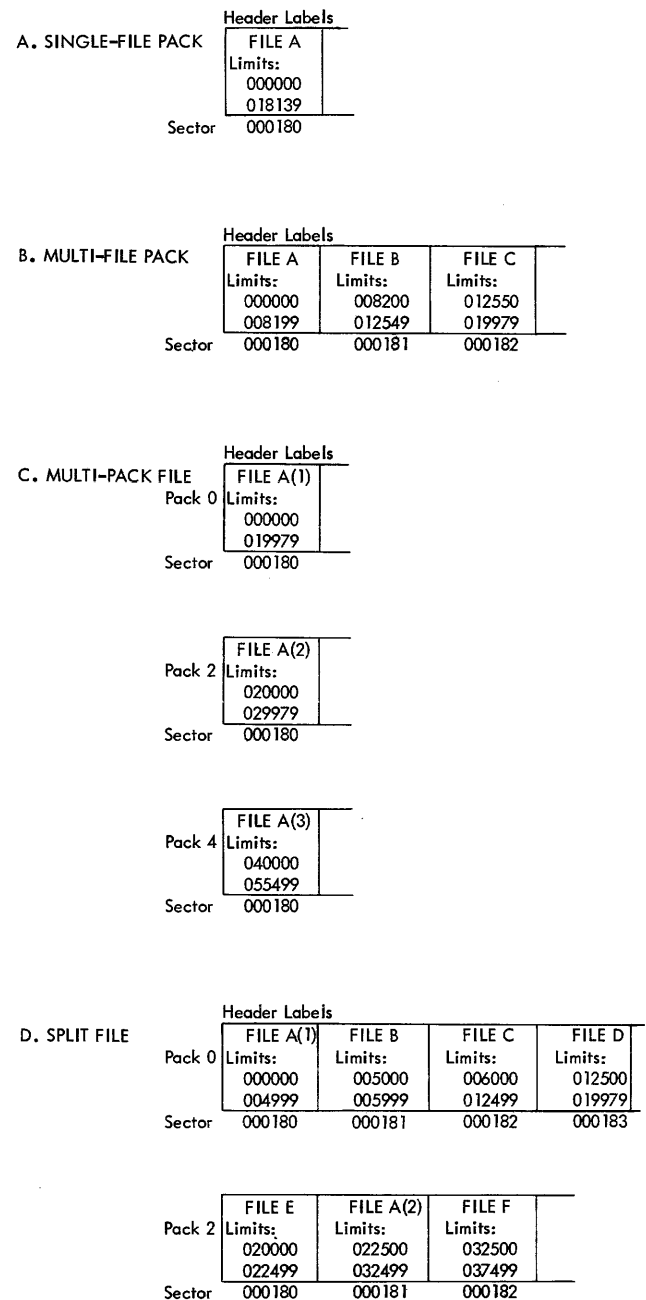
Figure 19. Schematic of Header-Label Arrangement for Files in the IBM 1311
