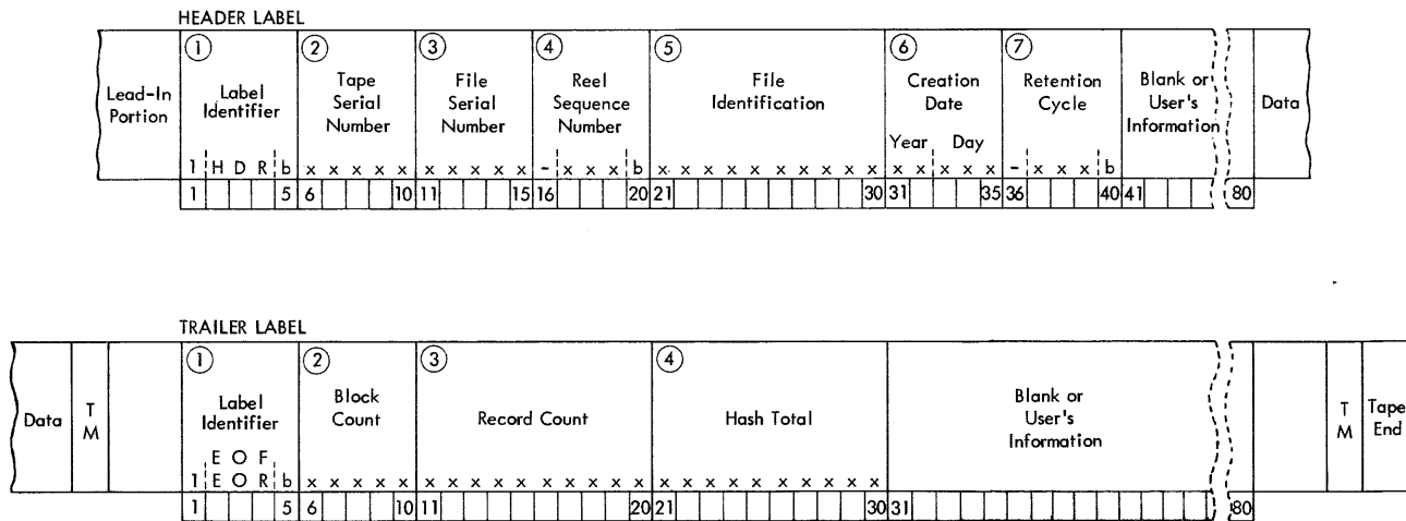
Figure 22. Schematic of Standard 80-Character Tape Label Fields Processed by IOCS (Type B)
